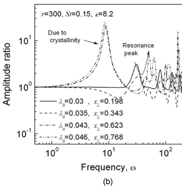
Fig. 4. Effect of relaxation time on (a) leading eigenmode and (b) frequency response in low-speed spinning process.
