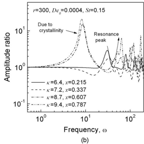
Fig. 5. Effect of FIC enhancement factor on (a) leading eigenmode and (b) frequency response in low-speed spinning process.
